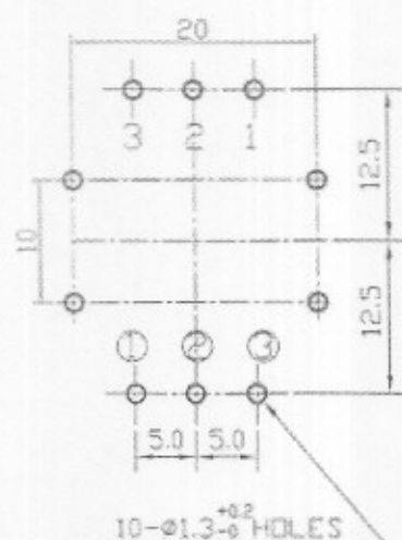
P.C.B. MOUNTING HOLE DETAIL
